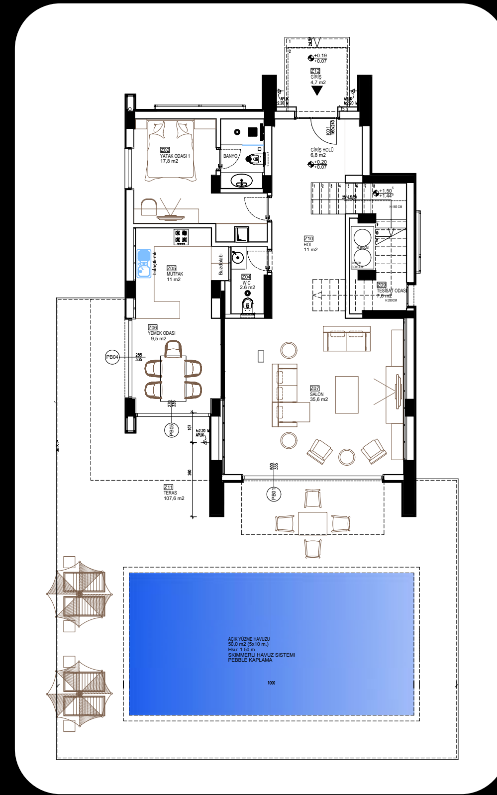
FIRST FLOOR
